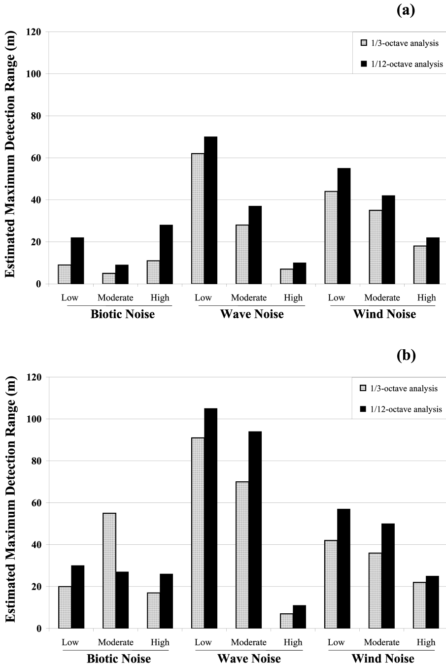
Figure 2. Estimated maximum detection range radii (m) for (a) representative pup 'female attraction call' or 'FAC' and (b) female 'pup attraction call' or 'PAC' in nine natural ambient noise conditions based on 1/3-octave (stipled bars) and 1/12-octave band (black bars) signal and noise analyses.
